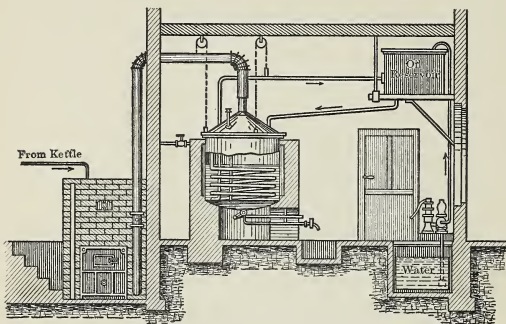
FIG. 8.—Lehmann's Apparatus.
